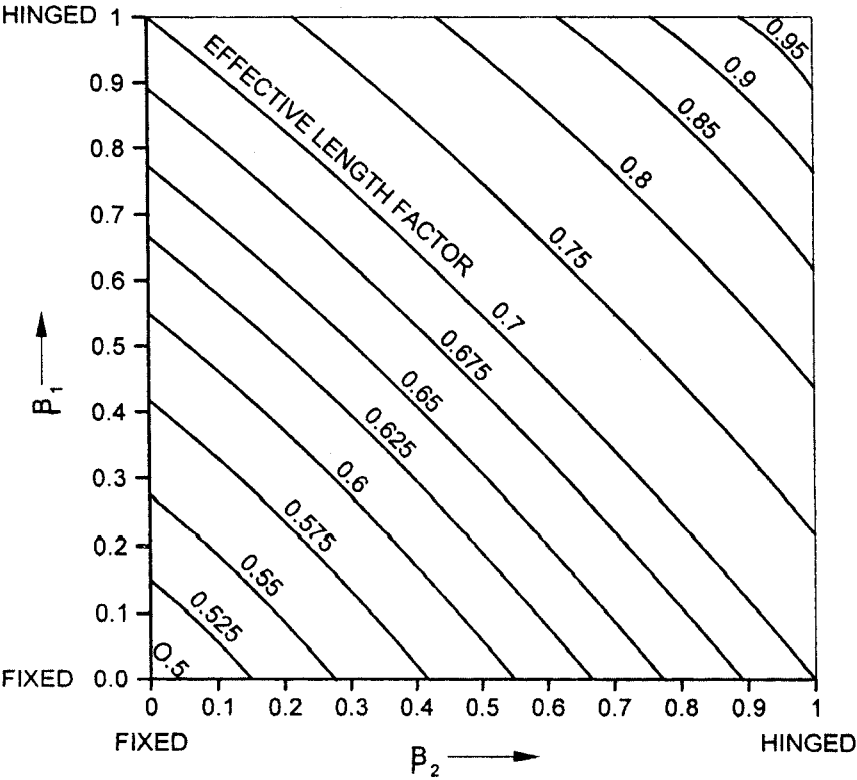
FIG. 27 COLUMN EFFECTIVE LENGTH FACTOR — NON-SWAY FRAME
