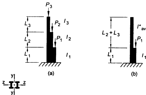
FIG. 29 EFFECTIVE LENGTH OF DOUBLE STEPPED COLUMNS
