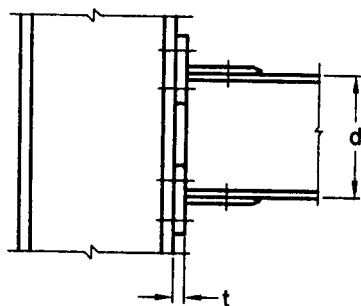
32G T-Stub
