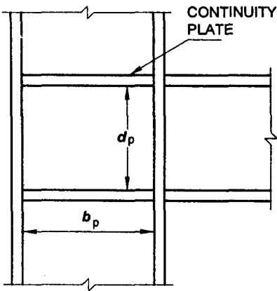
FIG. 21 CONTINUITY PLATES
