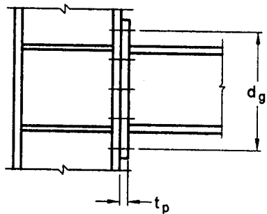
32F End Plate with Column Stiffeners
