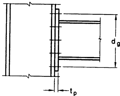
32E End Plate without Column Stiffeners
